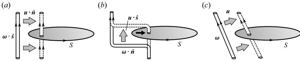
Figure 3. Advection of vortex filaments across the boundary of a stationary reference surface. (a) Advection of normal vorticity in the tangential direction, (\omega \cdot \hat{s})(u \cdot \hat{n}) . (b) Advection of tangential vorticity in the normal direction, (\omega \cdot \hat{n})(u \cdot \hat{s}) . (c) Advection of an oblique vortex filament across the boundary.
